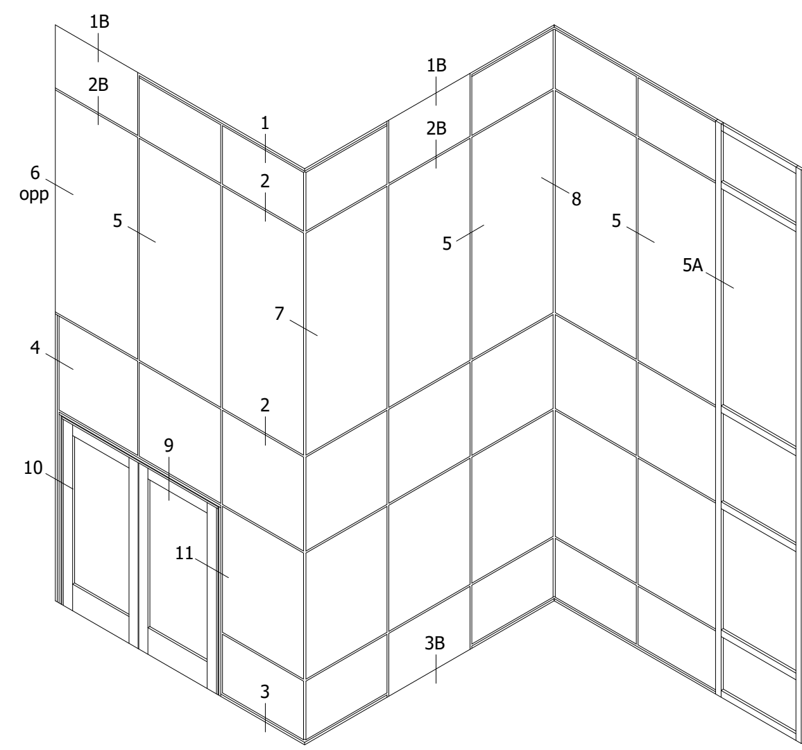
TYPICAL ELEVATION
