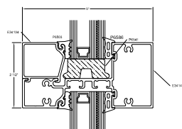
DRY GLAZE DETAIL
