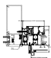
3 FLATBACK INSTALLATION STANDARD
