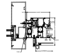
3B SF INSTALLATION OPTIONAL
