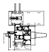
1A HEAD CURTAIN WALL INSTALLATION OPTIONAL
