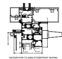
1B HEAD SF ADAPTOR OPTIONAL
