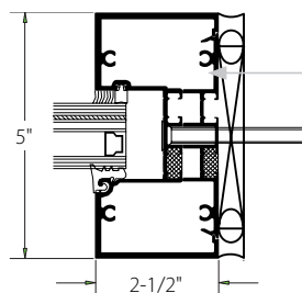
Screw Spline Frame Construction
