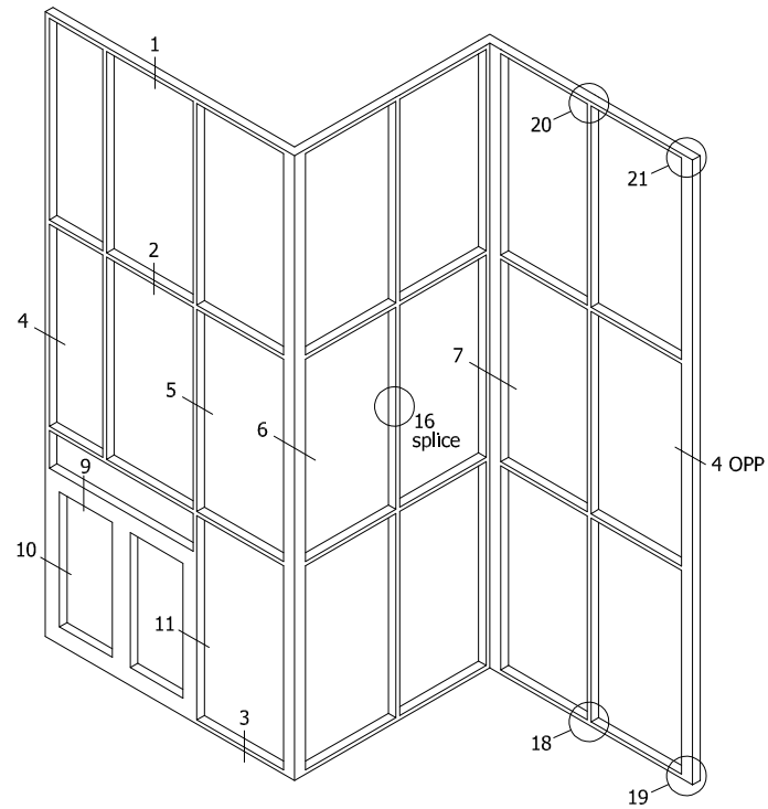
TYPICAL ELEVATION
