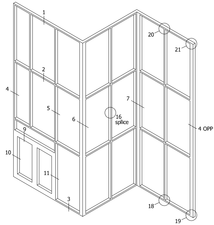
TYPICAL ELEVATION
